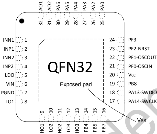
图 3-1 QFN32 Pinout1 PY32MD310K1xU7 (Top view)
