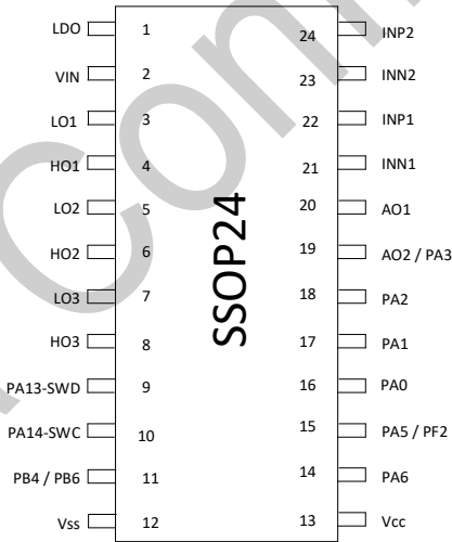
图 3-2 SSOP24 Pinout1 PY32MD310E1xM7 (Top view)
